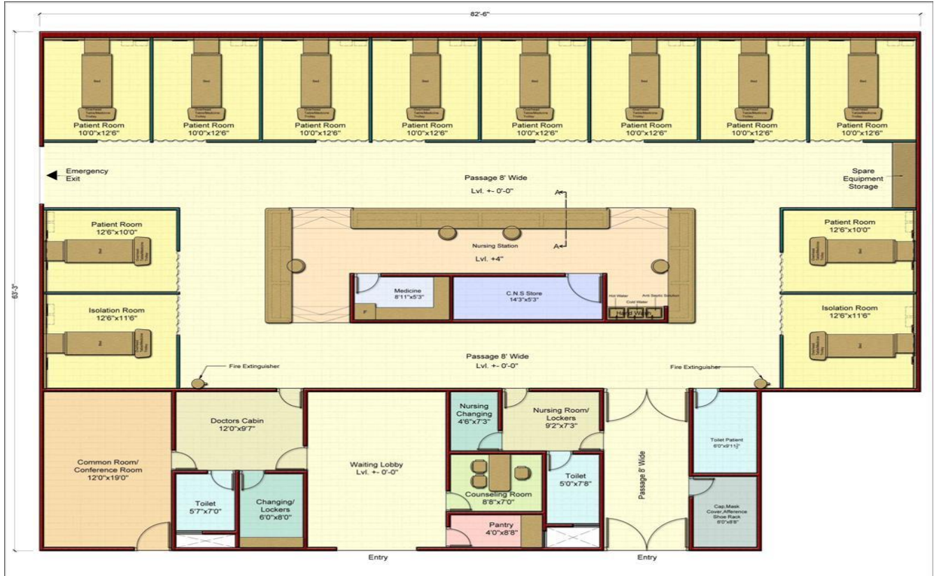
ISCCM ICU - 3 D view & Layout plan of ICU - 4
